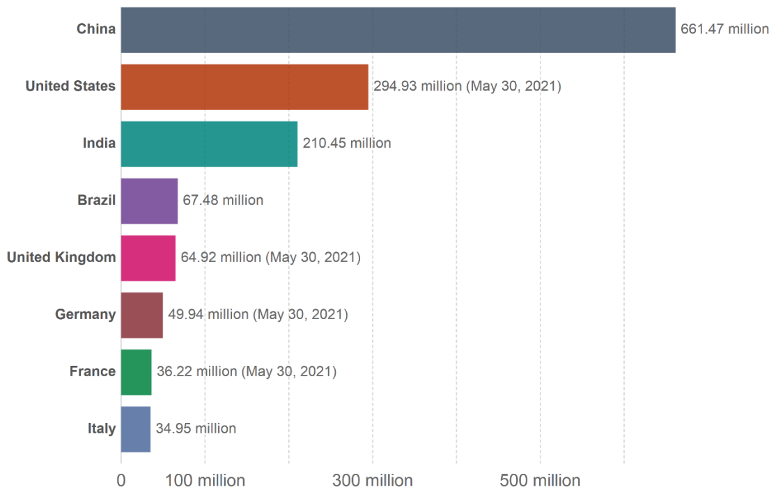
Source: Official data collated by Our World in Data – Last updated 1 June, 10:30 (London time)
