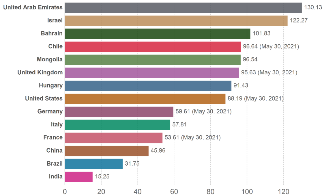
Source: Official data collated by Our World in Data – Last updated 1 June, 10:30 (London time)
